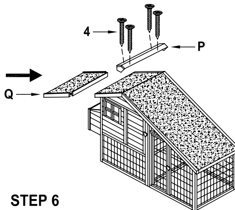
Use screw (4)*4 pcs to assemble the ridge. fix the nest roof on it is right position.
