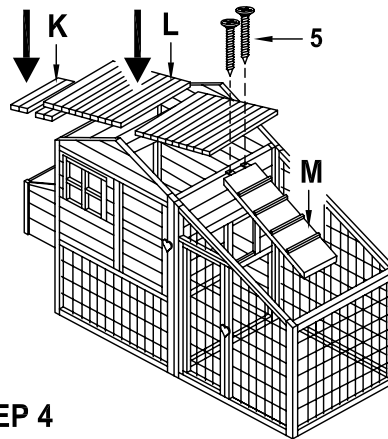
Place the nest floors, floors to their positions, place the ladder in the run, and use screw (5)*2pcs to fix the ladder with right panel.
