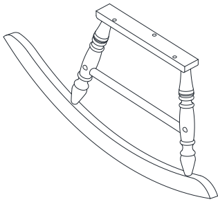
RIGHT LEG (C2) 832 x 380 x 49 mm
