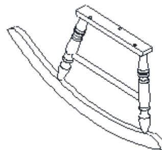
LEFT LEG (C1) 832 x 380 x 49 mm
