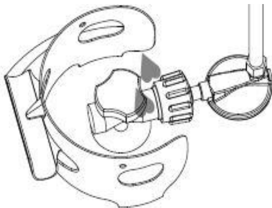
cylinder-regulator connection (Figure 18)
