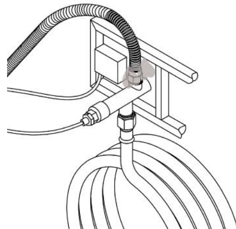
gas valve-bellows connection (Figure 19)
