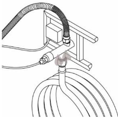
gas valve-hose connection (Figure 20)
