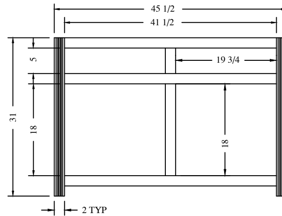
BACK PANEL (1/8 OKUME) (1) 33 1/2 X 20 1/4 (2) 15 1/4 X 27 1/2
